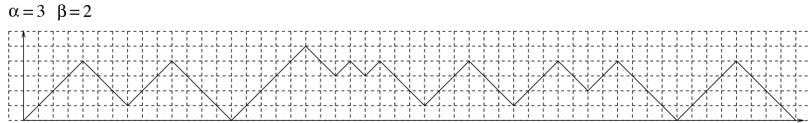
FIGURE 6. A Dyck D path with Val(D) = (2, 0) .
